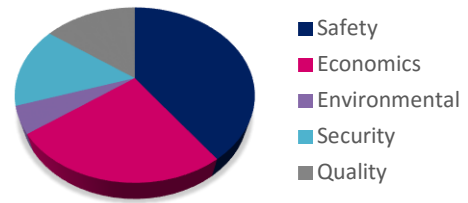
Classification Report
